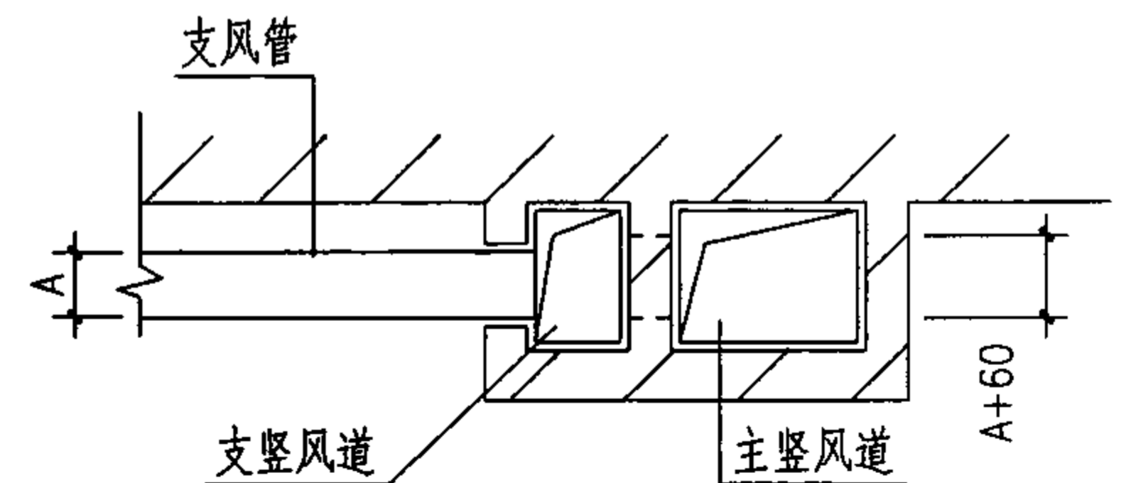
III-III
